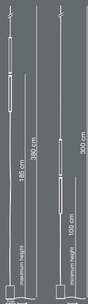
Equilibrio Floor
